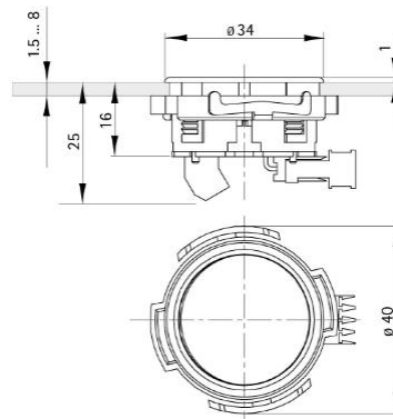
DIMENSION
