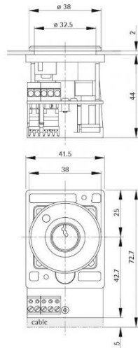
DIMENSION
