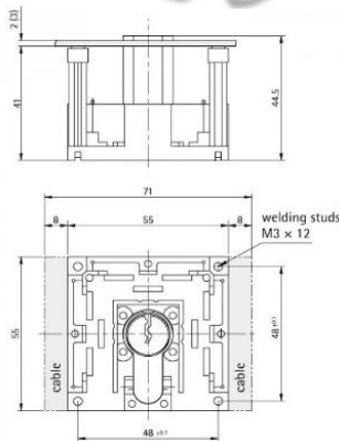
DIMENSION
