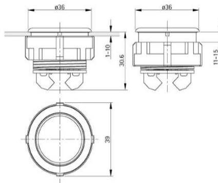
DIMENSION
